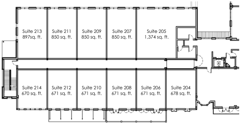
Second Floor/Office
