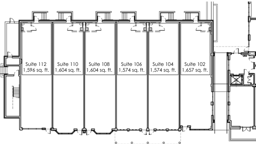
First Floor/Retail
